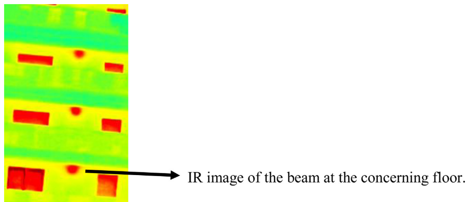
Fig. 19. Beam wall thermogram from outside.
