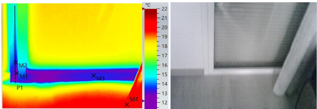
Fig. 24. Left: Thermogram of door window and the real image on the right.
