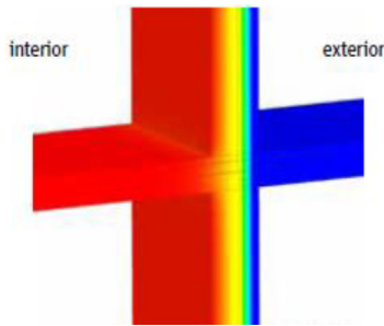
Fig. 3. Heat flow with thermal break.
