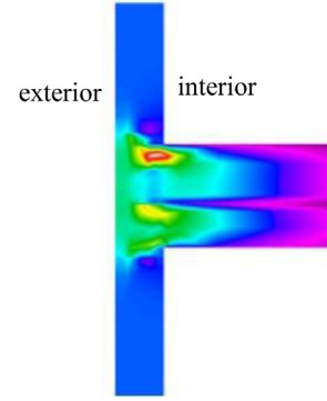
Fig. 4. Embedded beam in a wall.
