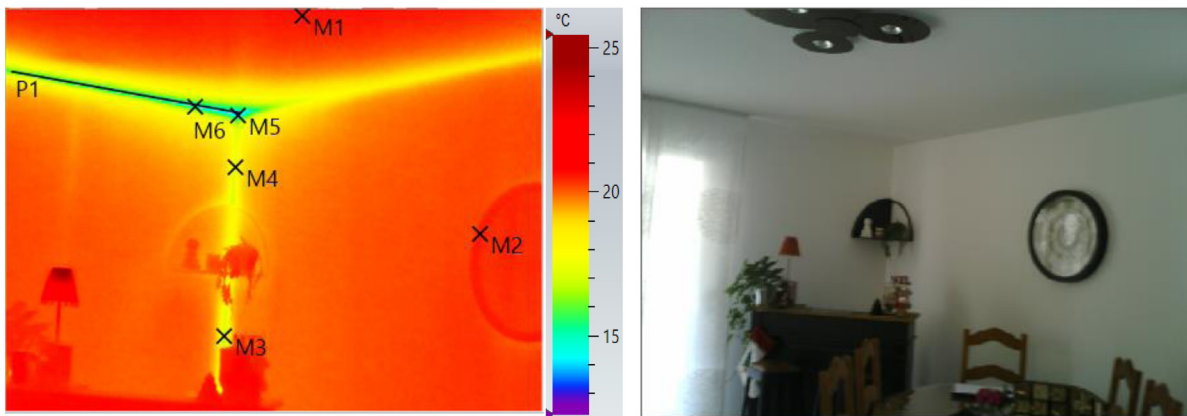
Fig. 12. Balcony wall thermal bridge on the left and real image on the right.
