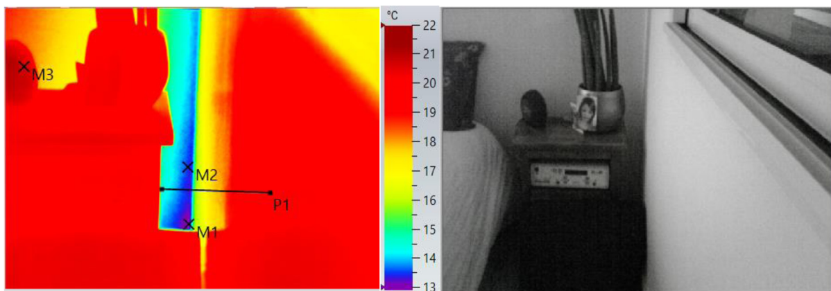
Fig. 9. Lower part of the wall to wall thermal bridge.
