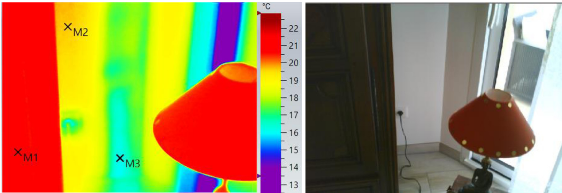
Fig. 21. Thermogram of the zone of missing insulator and the real image on the right.
