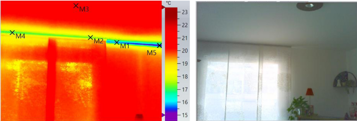
Fig. 14. Left: Balcony thermal bridge along the yellow line. The real image on the right.
