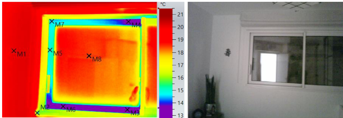
Fig. 22. Window thermogram on the left and real image on the right.
