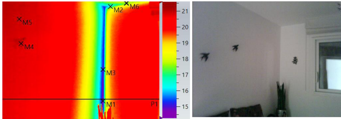
Fig. 7. Left is the thermogram of a wall to wall thermal bridge and real image on the right.
