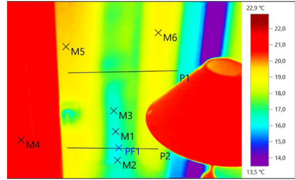
Fig. 1. Example of a thermal image.
