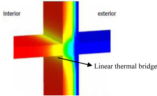
Fig. 2. Heat flow through balcony slab.
