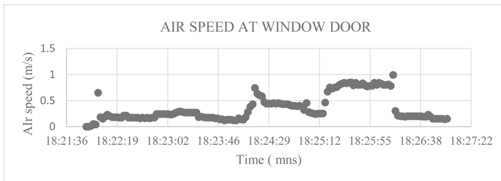
Fig. 28. Measuring air speed at the window door facing the north west.
