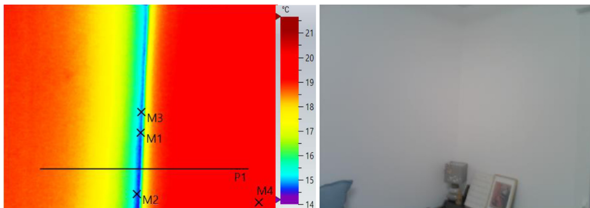
Fig. 11. On the left, another wall to wall thermal bridge and the real image on the right.
