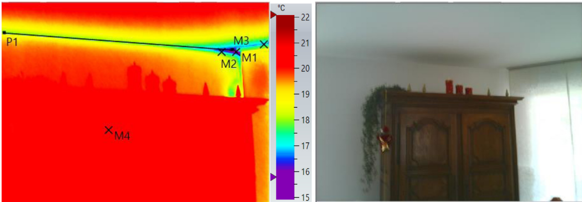
Fig. 15. Left: Thermograms between yellow and clear blue lines. Real image on the right.
