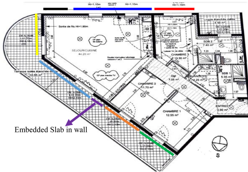
Fig. 6. Architectural plan of the apartment in the case study building.
