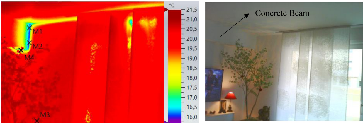
Fig. 20. Thermogram and real image of the slab wall junction.
