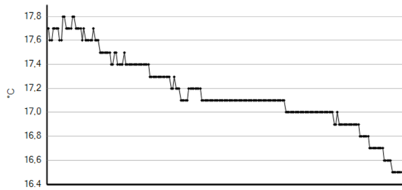
Fig. 18. Temperature profile along the thermal bridge in the thermogram.
