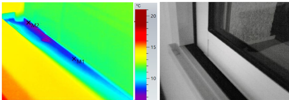
Fig. 23. Left: Air leakage at the lower part of the window. Real image on the right.
