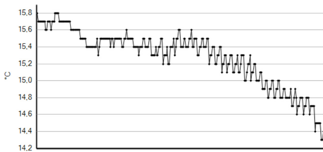
Fig. 13. Temperature profile in the thermal bridge in the IR image.
