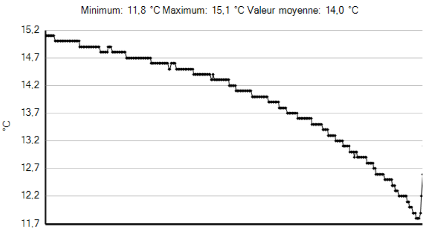
Fig. 25. Temperature profile at P1 in the thermogram.
