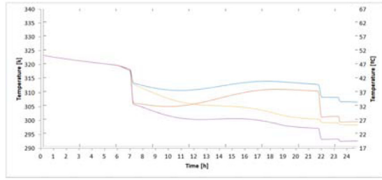
Fig. 22. Evolution of the temperature of the water inside the tank with (blue and yellow) and without (orange and purple) PHE for July and January respectively (Montalegre).
