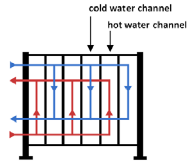
Fig. 5. Typical PHE configuration.
