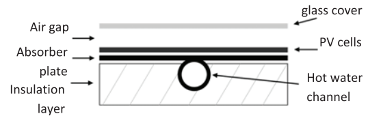
Fig. 2. Schematic of a typical PVT panel.
