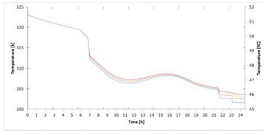
Fig. 15. Evolution of the temperature of the water inside the tank for SC1 (January), for each number of layers considered. Number of PCM layers: 6 (blue), 8 (orange), 10 (yellow) and 12 (purple).
