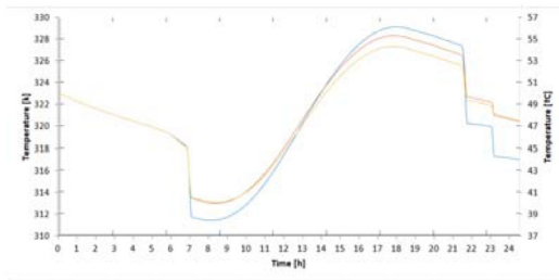
Fig. 16. Evolution of the temperature of the water inside the tank for SC1 (July), for each length of the PHE layers. Lengths: 0.4 [m] (blue), 0.8 [m] (orange) and 1.2 [m] (yellow).
