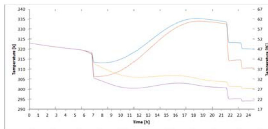
Fig. 21. Evolution of the temperature of the water inside the tank with (blue and yellow) and without (orange and purple) PHE for July and January respectively (Castelo Branco).
