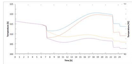
Fig. 19. Evolution of the temperature of the water inside the tank for SC1 (January), for each thickness of the PCM layer. Thicknesses: 0.007 [m] (blue), 0.014 [m] (orange) and 0.021 [m] (yellow).
