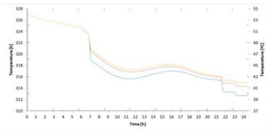
Fig. 13. Evolution of the temperature of the water inside the tank for SC1 (July), for each number of layers considered. Number of PCM layers: 6 (blue), 8 (orange), 10 (yellow) and 12 (purple).
