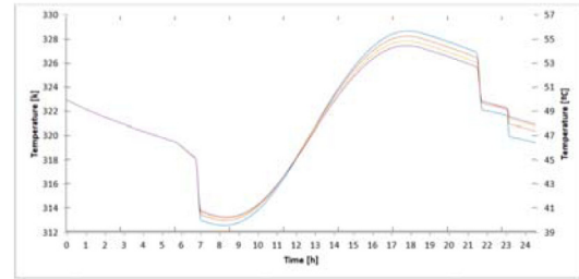
Fig. 14. Evolution of the temperature of the water inside the tank for SC1 (July), for each number of layers considered. Number of PCM layers: 6 (blue), 8 (orange), 10 (yellow) and 12 (purple).
