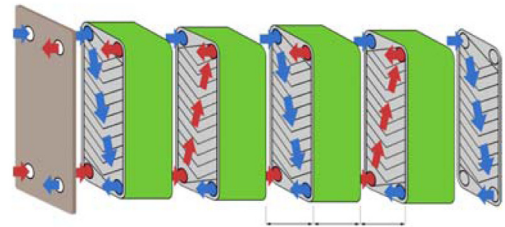
Fig. 3. Schematic of a PHE with PCM intercalated between a hot and a cold water channel.
