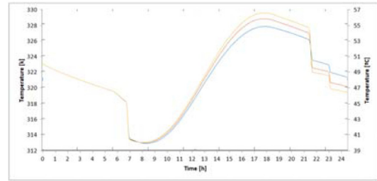
Fig. 18. Evolution of the temperature of the water inside the tank for SC1 (July), for each thickness of the PCM layer. Thicknesses: 0.016 [m] (blue), 0.031 [m] (orange) and 0.047 [m] (yellow).
