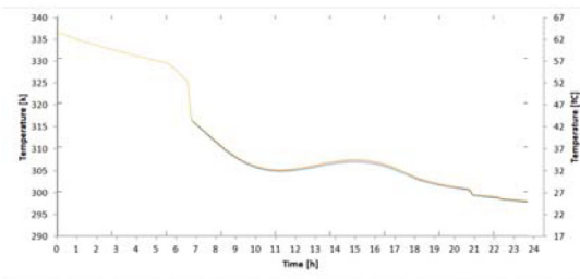
Fig. 20. Evolution of the temperature of the water inside the tank with (blue and yellow) and without (orange and purple) PHE for July and January respectively (Lisboa).
