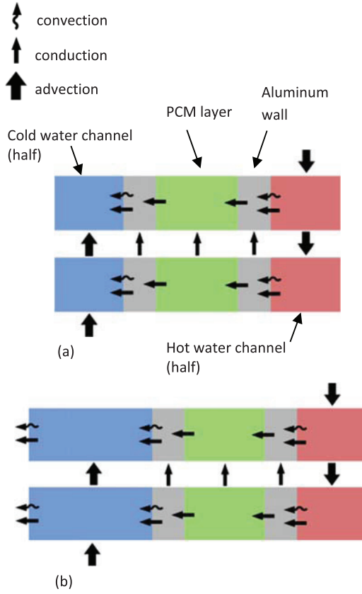
Fig. 9. Unit 1 (a) and Unit 2 (b).
