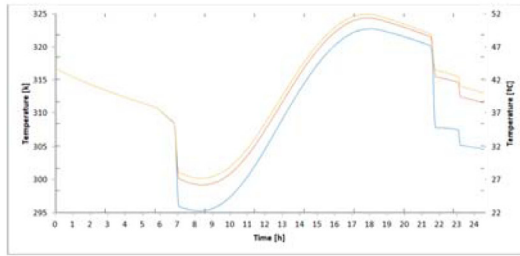
Fig. 12. Evolution of the temperature of the water inside the tank for SC1 (July), for each thickness of the cold water channel. Thicknesses: 0.05 [m] (blue), 0.1 [m] (orange) and 0.15 [m] (yellow).
