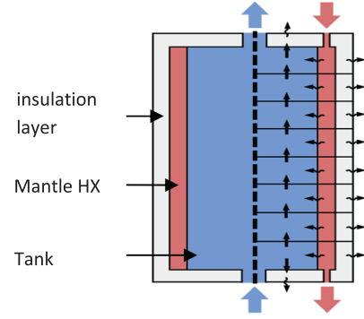
Fig. 11. Tank model.
