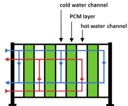
Fig. 6. Configuration of the PHE considered in this work.
