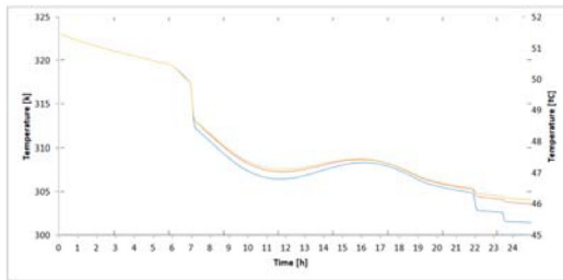
Fig. 17. Evolution of the temperature of the water inside the tank for SC1 (January), for each length of the PHE layers. Lengths: 0.4 [m] (blue), 0.8 [m] (orange) and 1.2 [m] (yellow).
